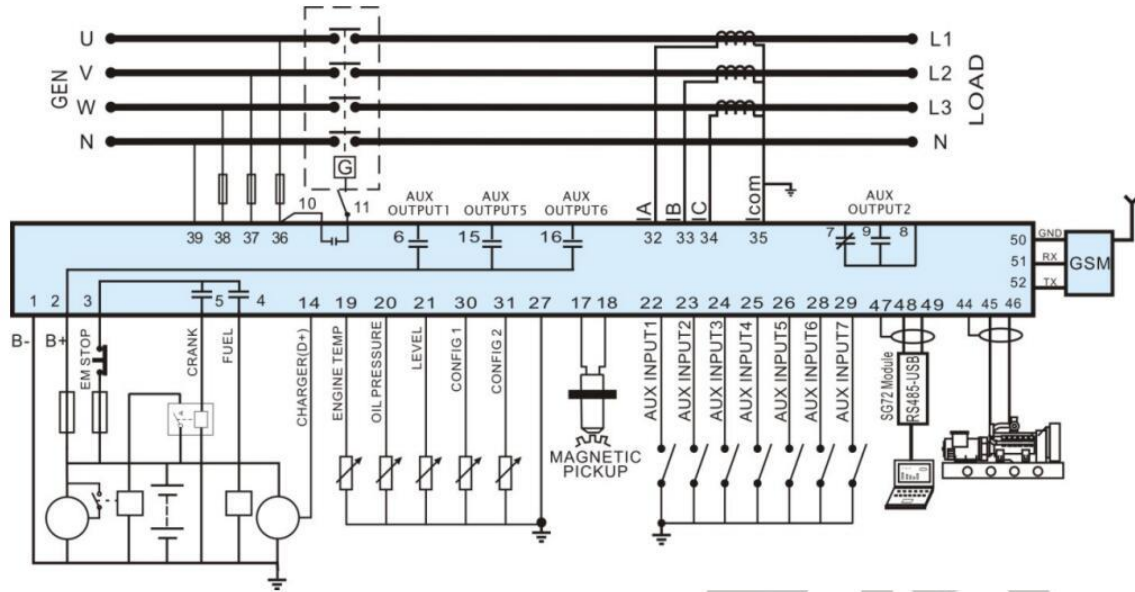
HGM7210CAN typical application diagram
